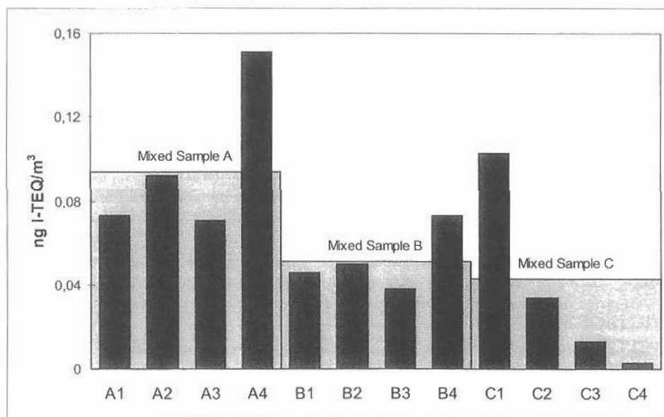
Figure 2. PCDD/F concentrations in weekly (1-4) and monthly mixed (A-C) samples from the waste wood combustion plant; ng I-TEQ/m 3 refer to 0 °C, 101.3 kPa, dry, related to 11 % O 2
