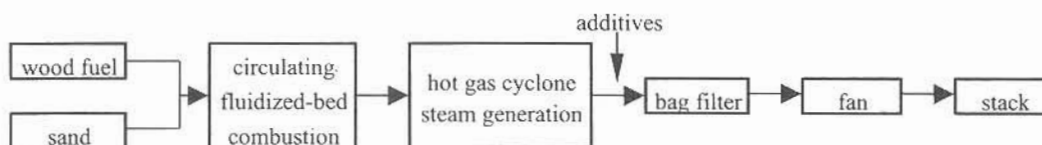
Figure 1. Description of the firing and flue gas cleaning of the waste wood combustion plant.
