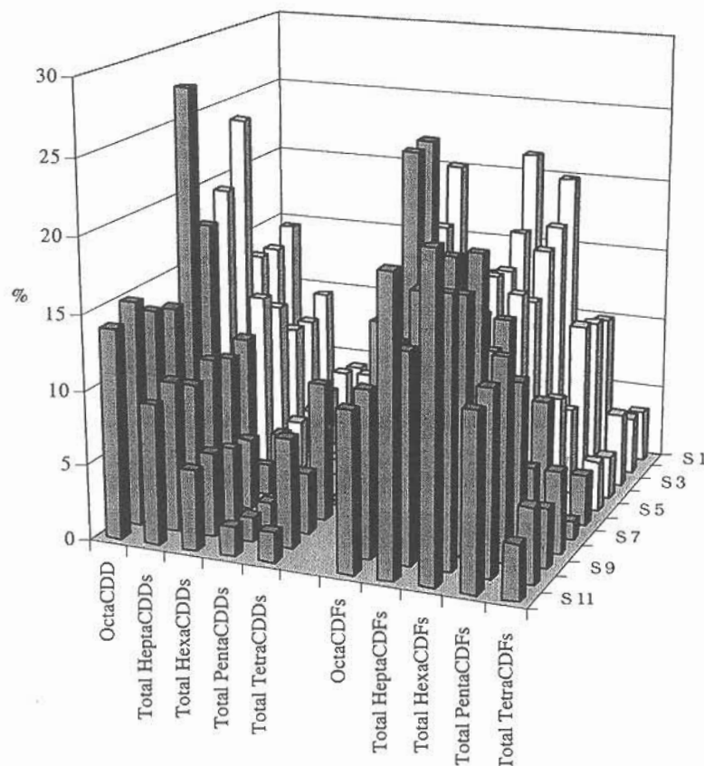
Fig. 2: Proportional parts of Tetra- through OctaCDF/Ds in the flue gas samples taken during higher (1,200 °C, light columns) and lower (1,000 °C, dark columns) incineration temperatures
